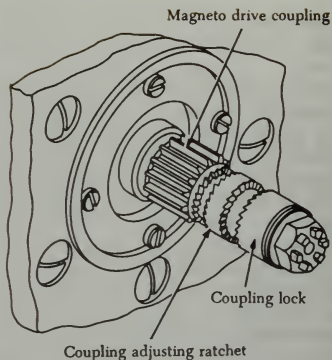
FIGURE 4-43. Magneto ratchet arrangement.
